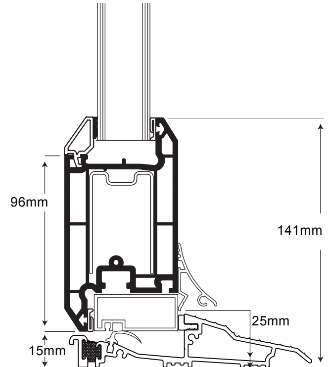
Secured by Design Threshold Proline AM3 Threshold (Open in)
